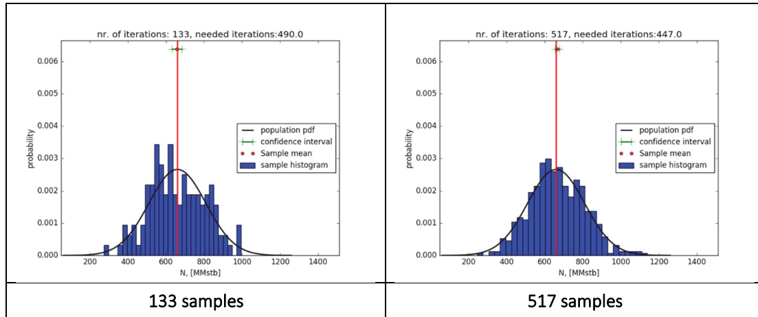
FIGURE 5-6. PROBABILITY DISTRIBUTION OF INITIAL OIL IN PLACE SAMPLED FROM A NORMAL DISTRIBUTION FOR DIFFERENT NUMBER OF SAMPLES
