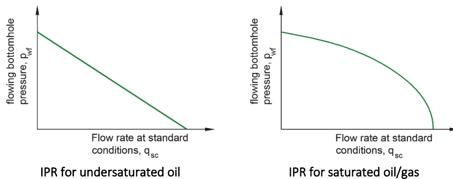
FIGURE 2-3. IPR CURVE
