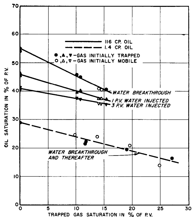
FIG. 5—RELATIONSHIPS BETWEEN TRAPPED GAS AND RESIDUAL OIL SATURATIONS, TORPEDO SANDSTONE CORES
