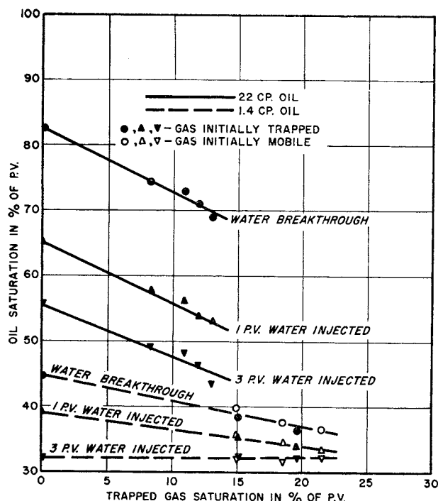
FIG. 6—RELATIONSHIPS BETWEEN TRAPPED GAS AND RESIDUAL OIL SATURATIONS, DRI-FILMED ALUNDUM CORE (DFA87).
