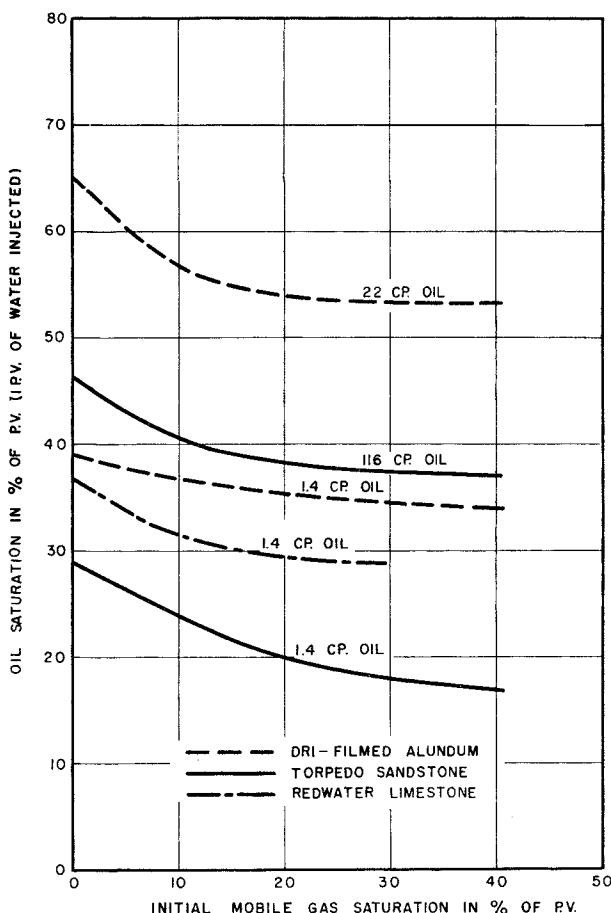
FIG. 7—RELATIONSHIPS BETWEEN INITIAL MOBILE GAS SATURATION AND RESIDUAL OIL SATURATION AFTER X 1 PV OF WATER INJECTION.
