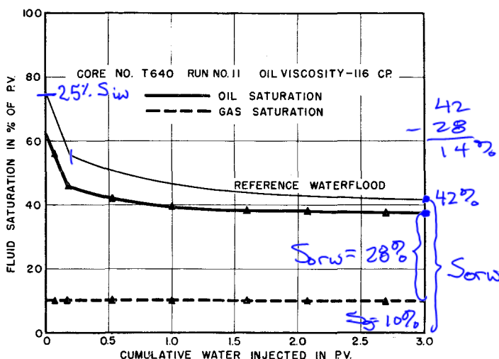
FIG. 1—WATER FLOOD IN THE PRESENCE OF TRAPPED GAS.
