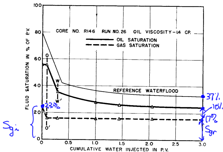
FIG. 2—WATER FLOOD IN THE PRESENCE OF INITIAL MOBILE GAS.
