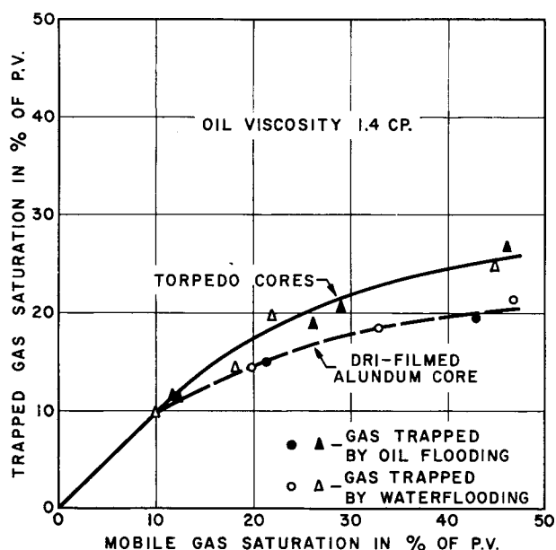
FIG. 4—DISPLACEMENT OF MOBILE GAS BY OIL AND WATER INJECTION.
