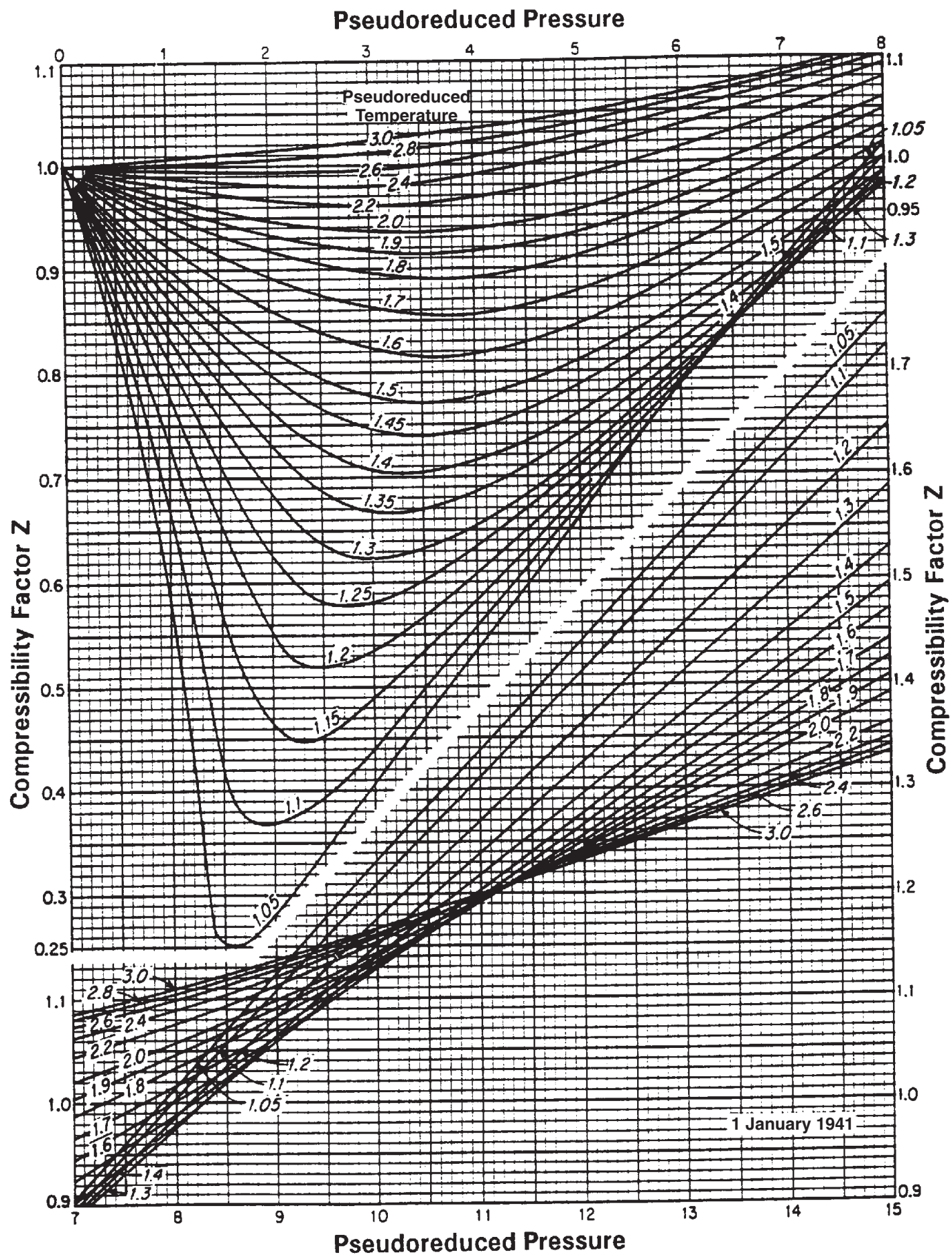
Fig. 3.6—Standing-Katz 4 Z-factor chart.
