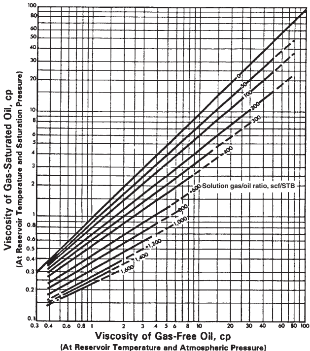
Fig. 3.22—Live-oil (saturated) viscosity as a function of dead-oil viscosity and solution gas/oil ratio (from Standing, 33 after Beal 72 correlation).
