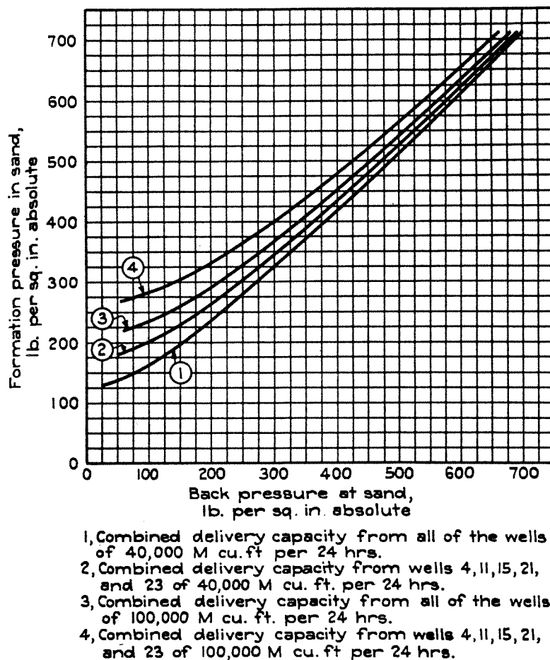
FIGURE 33.—Relationships between formation pressure and back pressure at the face of the sand for definite delivery rates from gas wells illustrated in figure 31
