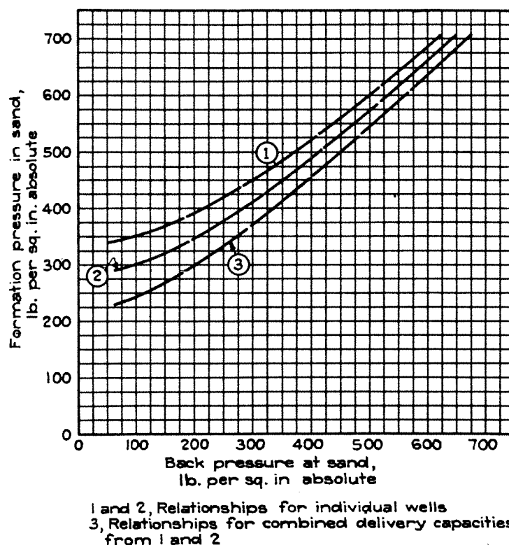
FIGURE 30.—Relationship between formation pressure and back pressure at the face of the sand for delivery of gas at definite rate from gas wells illustrated in figure 29
