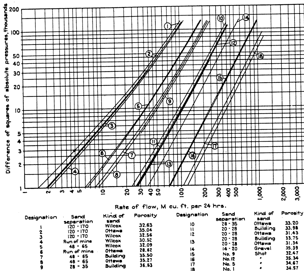
FIGURE 59.—Effect of grain size and shape on flow of gas through unconsolidated porous media
