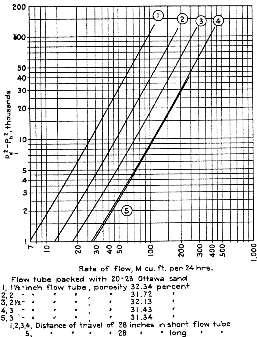
FIGURE 62.—Effect of diameter of flow tube on flow of gas through unconsolidated porous media
