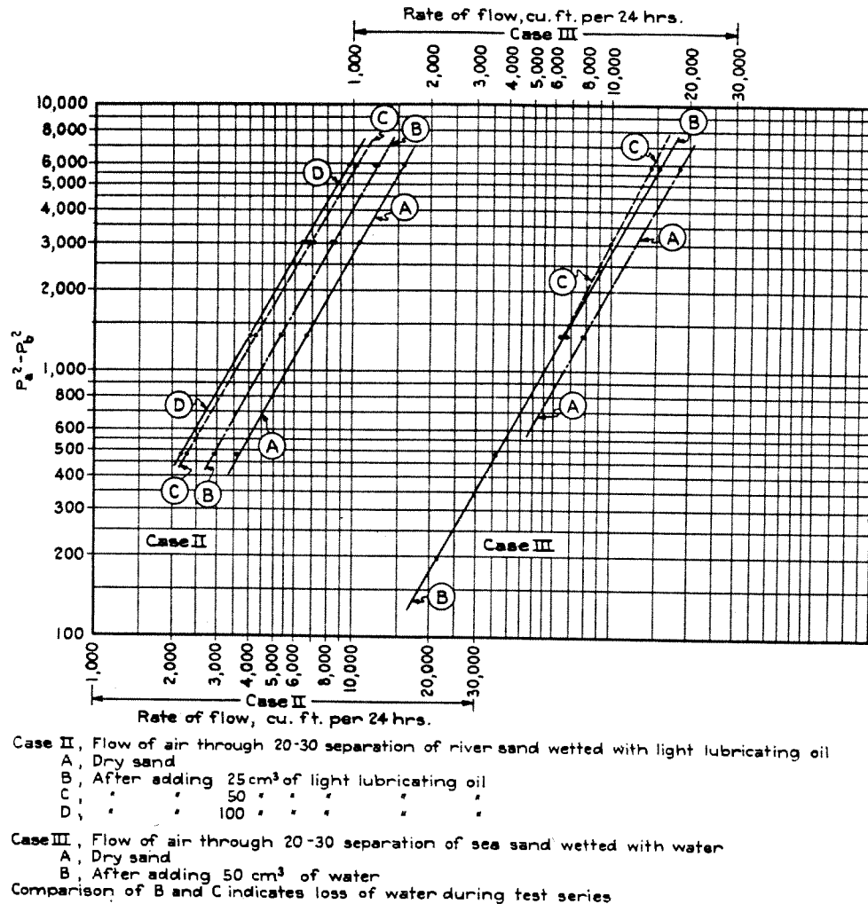
FIGURE 66.—Effect of liquid on flow of air through unconsolidated porous media, cases II and III
