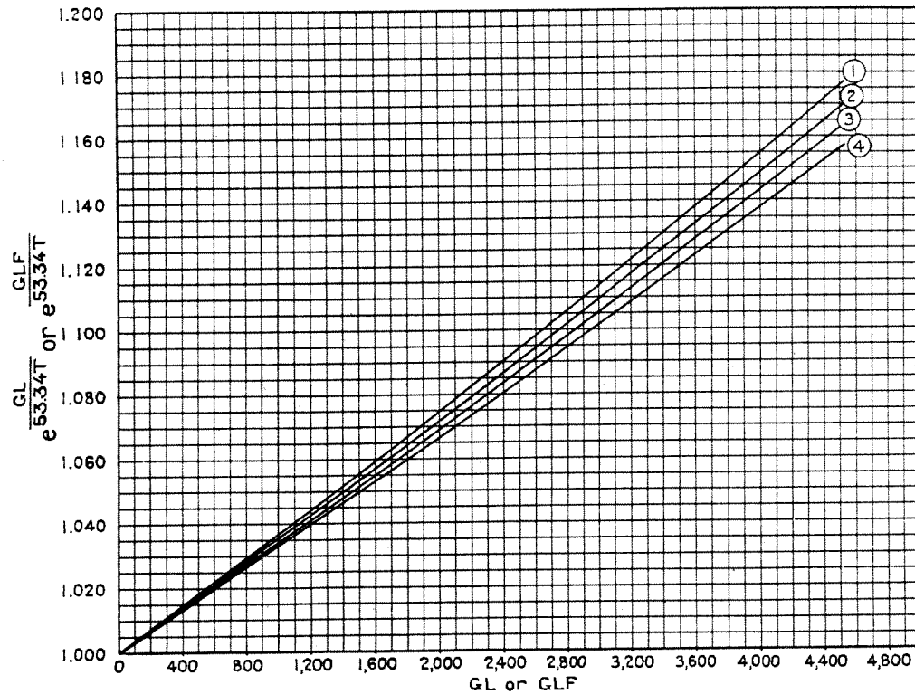
FIGURE 49.—Relationship between \frac{GL}{53.34T} and GL for different average temperatures in determining effect of deviation of gas from Boyle's law on pressure due to weight of column of gas
