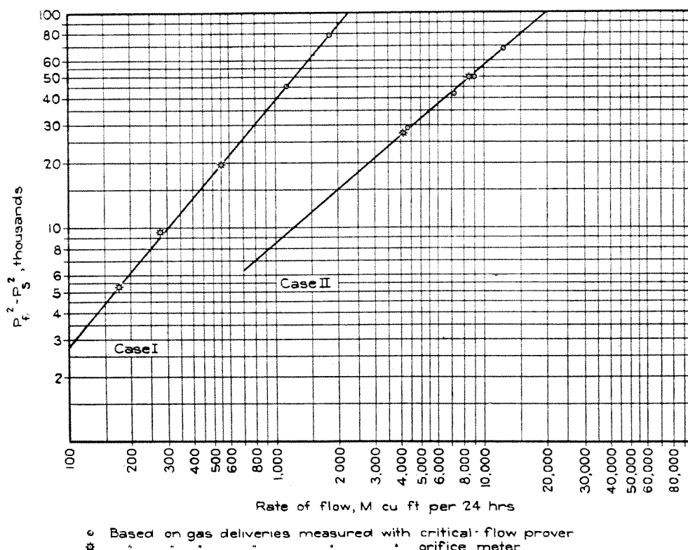
FIGURE 3.—Measurement of gas deliveries with critical-flow prover and orifice meter for same back-pressure tests on natural-gas wells
