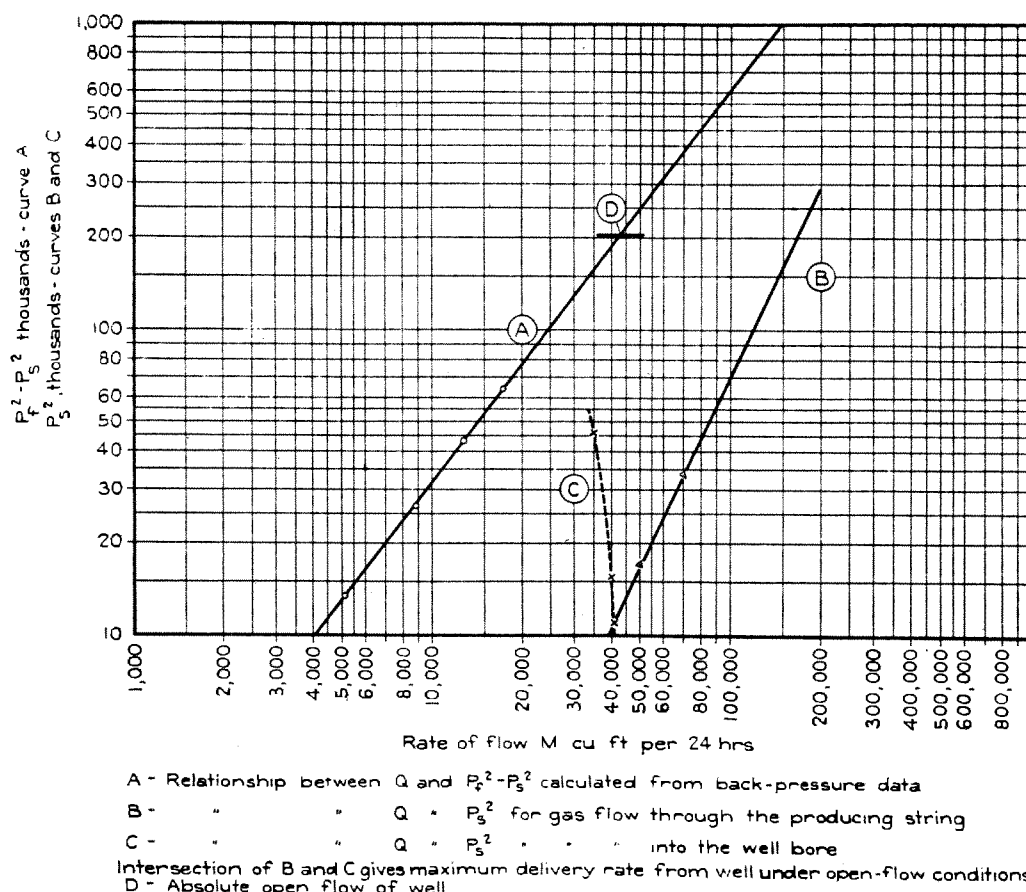
FIGURE 6.—Results of back-pressure test on a natural-gas well
