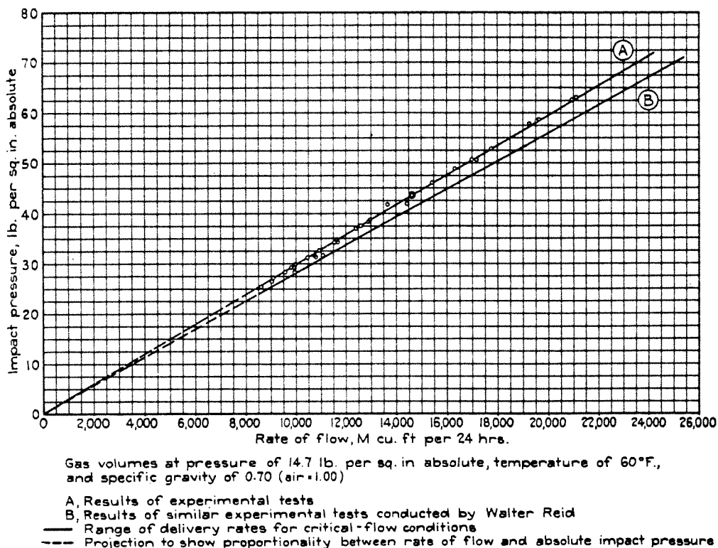
FIGURE 41.—Relationship between impact pressure and delivery rate of gas for critical flow with tip of Pitot tube at center of discharge opening of pipe
