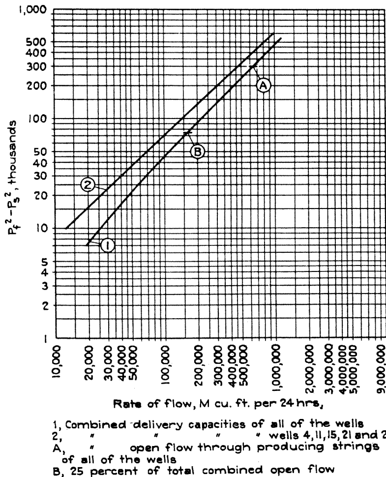
FIGURE 32.—Combined delivery capacities of gas wells illustrated in figure 31
