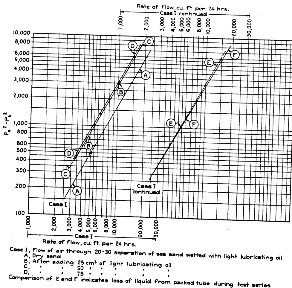
FIGURE 65.—Effect of liquid on flow of air through unconsolidated porous media, case I
