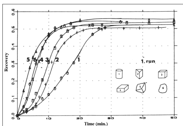
Fig. 4 Effect of size and shape on imbibition oil recovery (from Torsæter and Silseth 28 )
