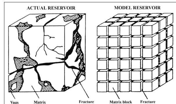
Fig. 1 Idealization of a fractured system (from Warren and Root 2 )
