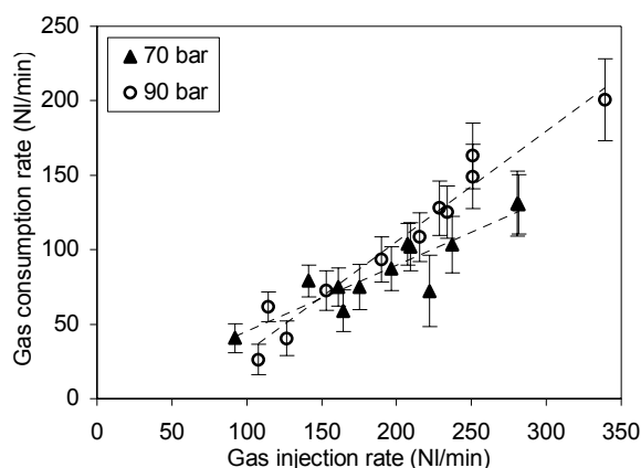
Figure 3 Methane gas consumption rate as a function of gas injection rate at 70 and 90 bar at 7 °C.
