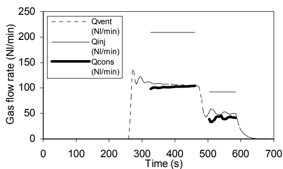
Figure 2 Experiment 3a at 70 bar and 7.2 °C. Methane gas. The gas injection rate was changed after about 460 seconds.
