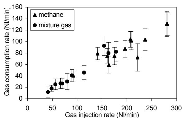
Figure 5 Gas consumption rate as a function of gas injection rate for methane gas and natural gas mixture. Pressure is 70 bar, and subcooling is approximately 3 °C in experiments with both gas compositions.
