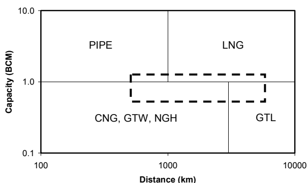
Figure 5 - Capacity-distance diagram (BCM per year versus km).
