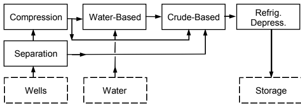
Figure 3 Main units of a hydrate slurry process.
