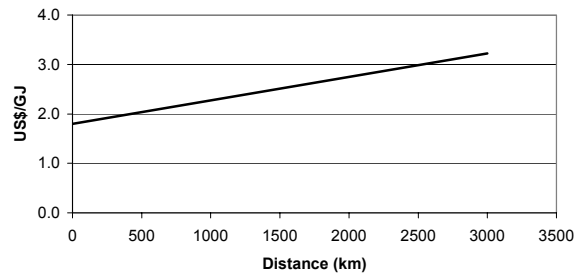
Figure 4 - Approximate transport cost of 50 MMscfd natural gas as slurry-hydrate.
