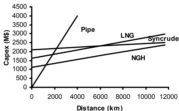
Figure 1 Approximate capital cost with transport distance, dry-hydrate case.
