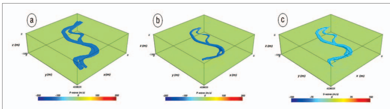
Figure 7. (a) Difference between base and monitor model for compressional-wave velocity showing the true time-lapse effect. (b) Compressional-wave velocity time-lapse effect inverted by EFWI. (c) Corresponding shear-wave time-lapse effect.
