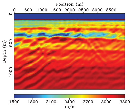
Figure 8. Acoustic FWI with \rho equal to the true model.
