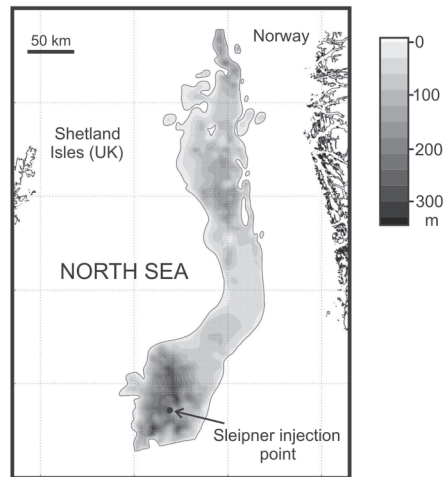
Figure 1. Location map showing Sleipner and the extent/thickness of the Utsira Sand aquifer.
